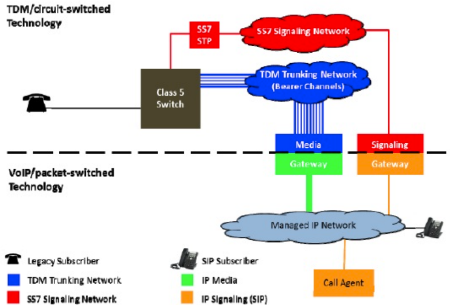
Figure 1: VoIP-to-TDM Interconnection
